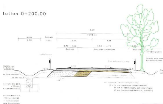
Typical cross-section of station 0+200
