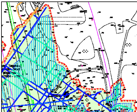
Extract from operation mining plan, pit Elvira, Lichterfeld
